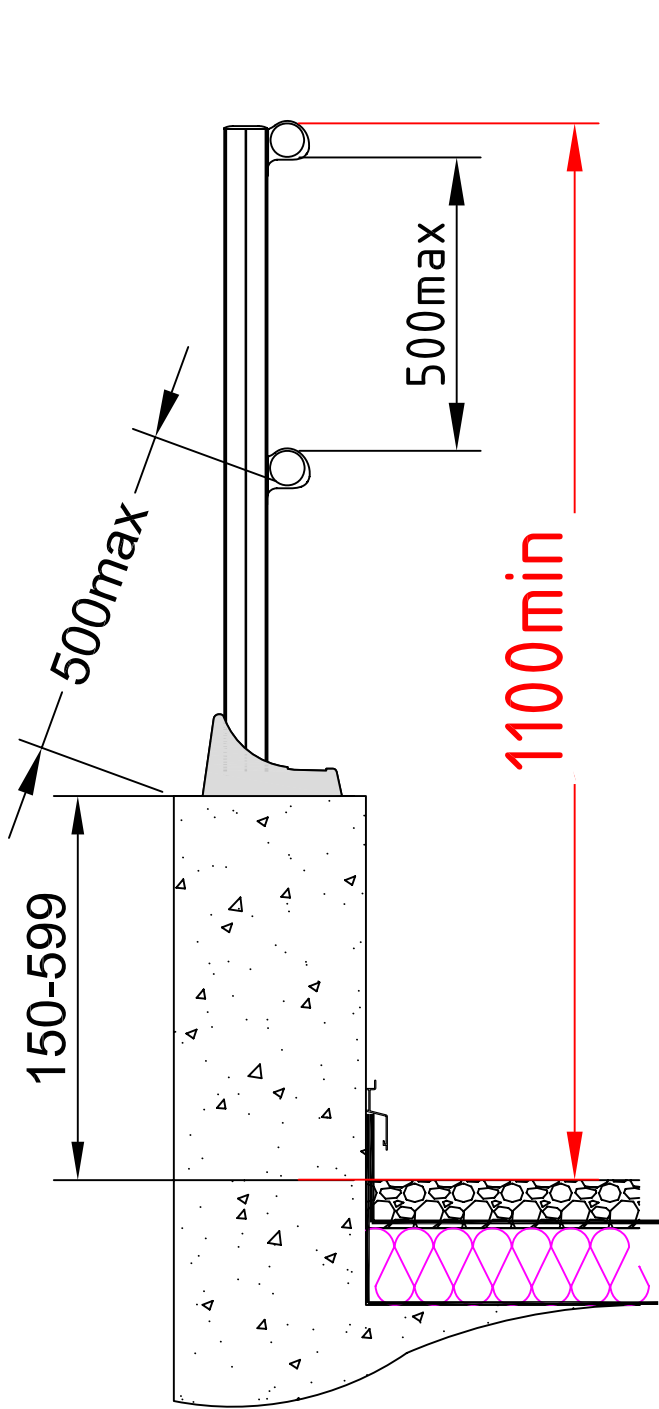
without plinth
