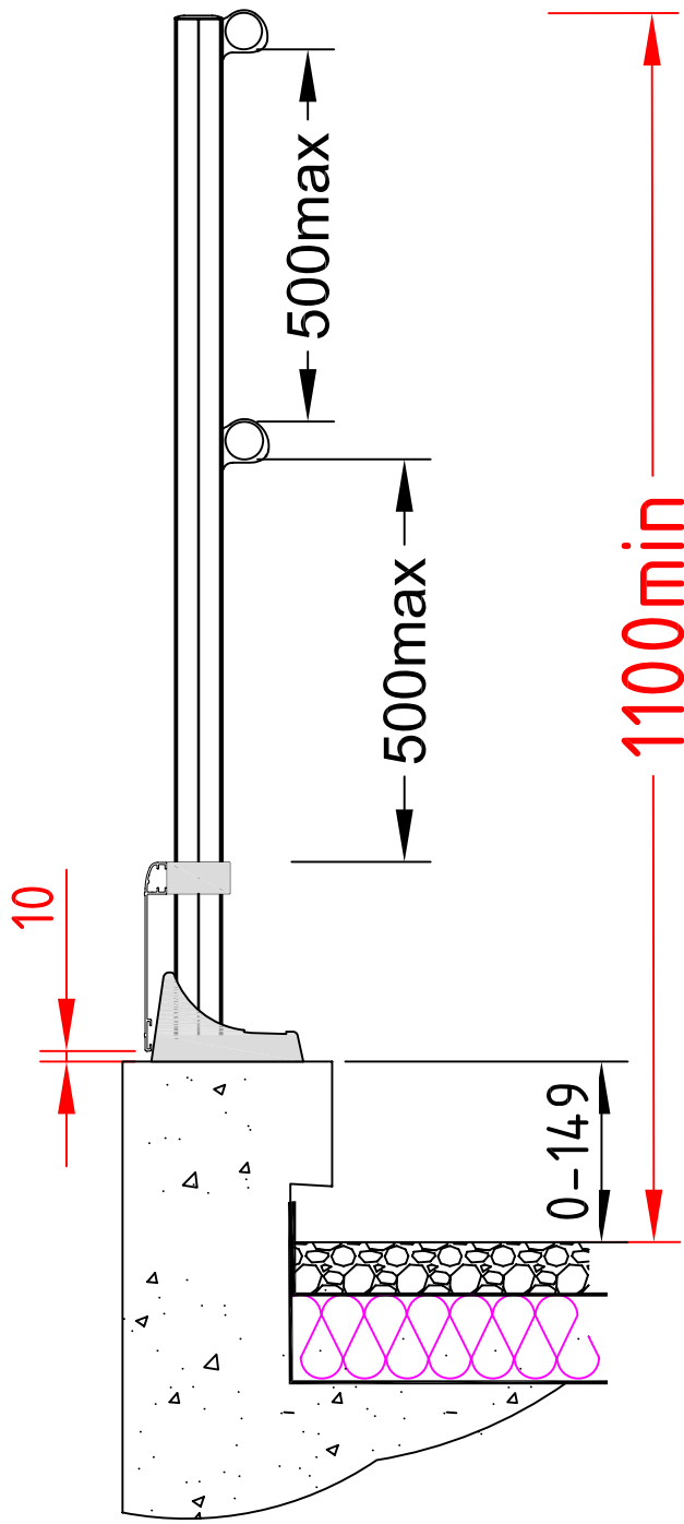
with plinth
