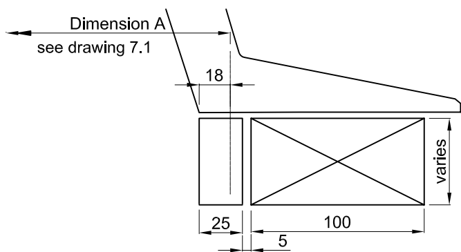
Typical dimensions for Rooflight with 240mm upstand
