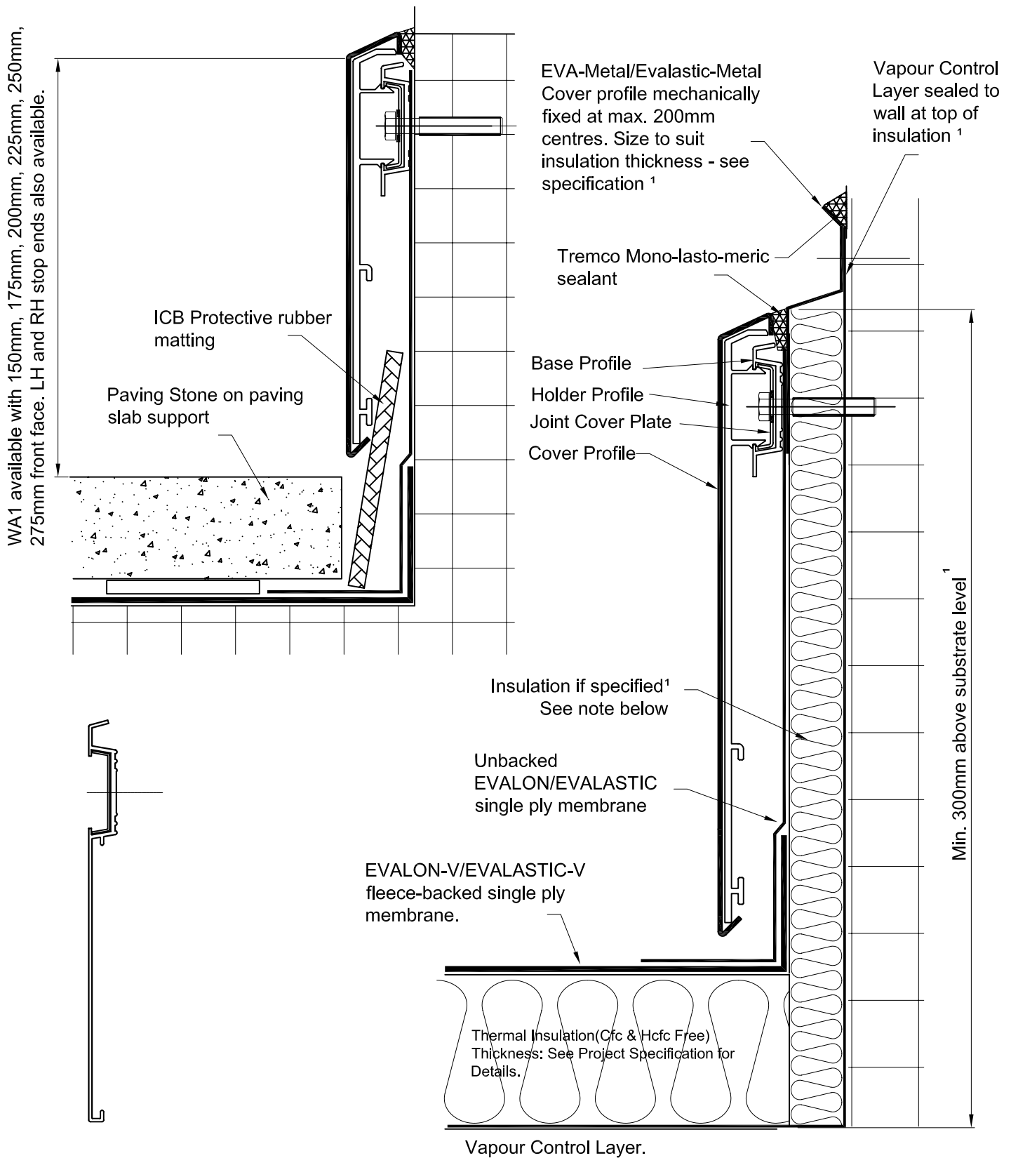
WA150 Skirting Profile
