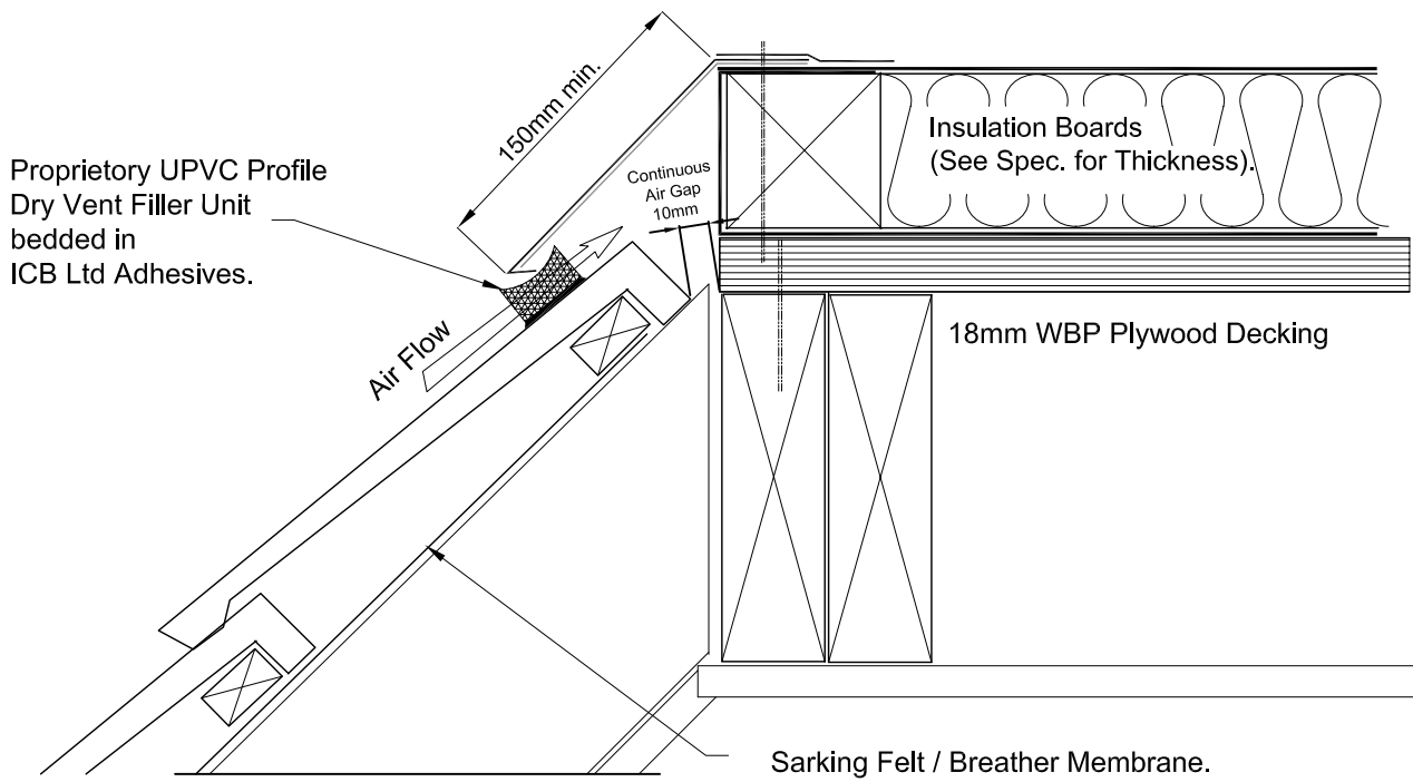
VENTED PITCHED ROOF JUNCTION
