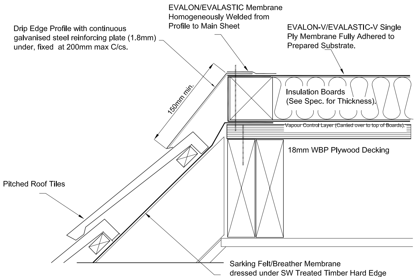
NON VENTED PITCHED ROOF JUNCTION
