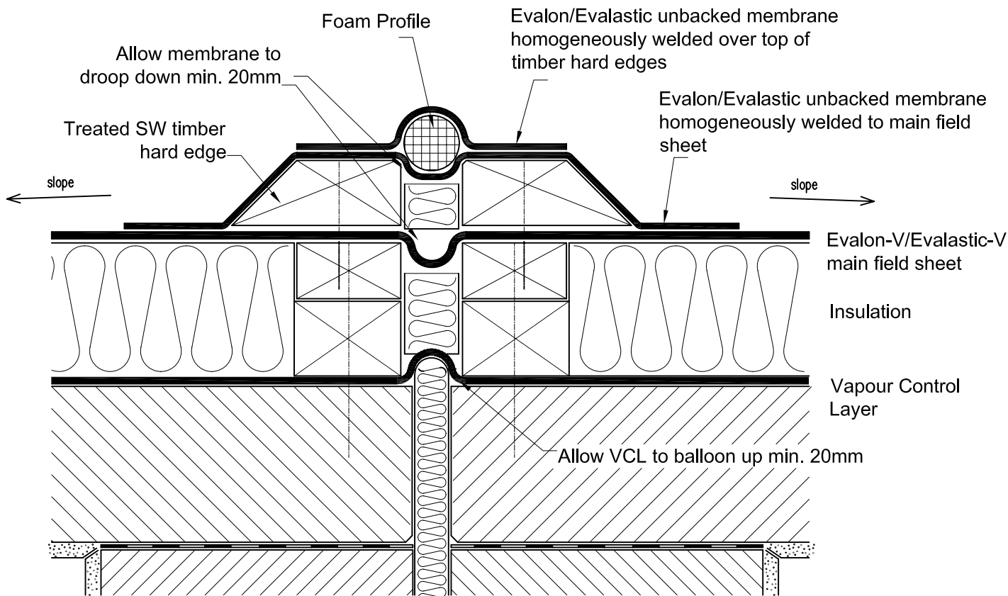
Typical expansion joint detail in Flat Roof
