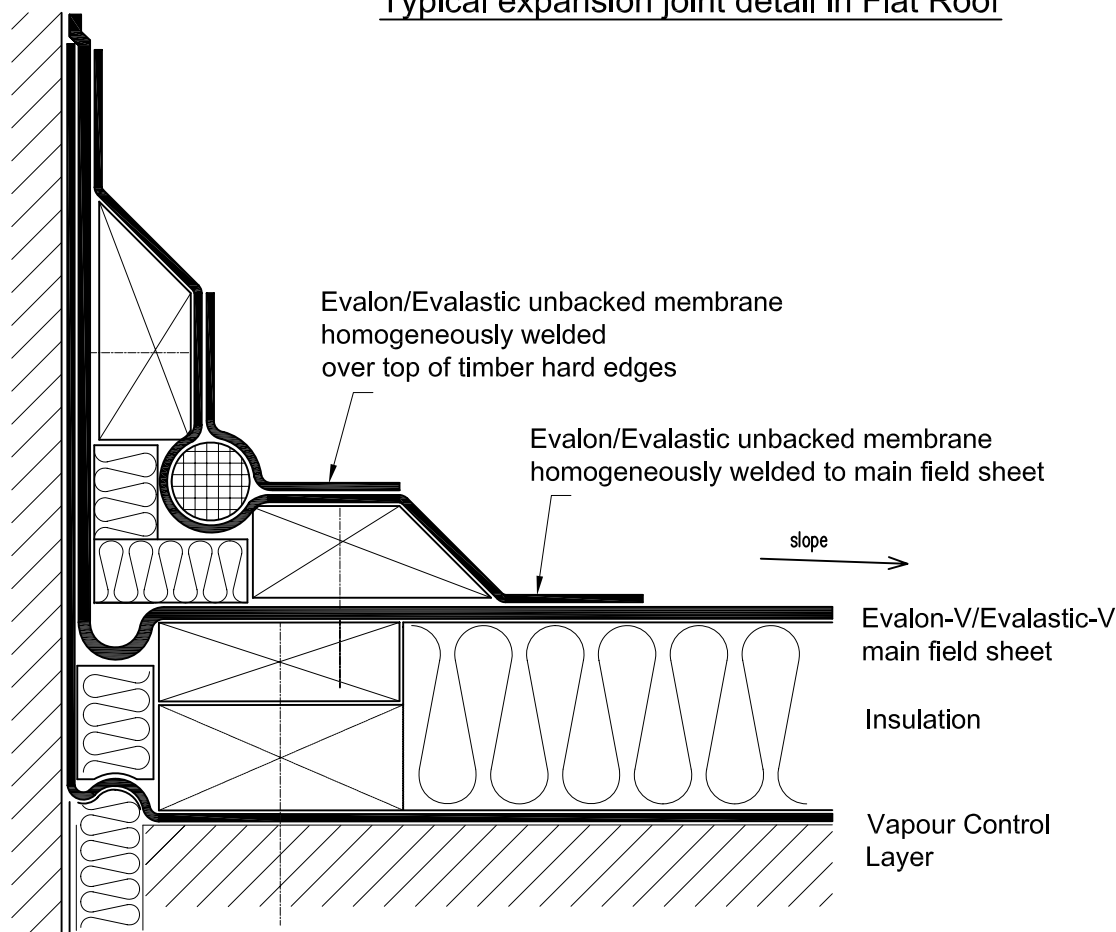
Typical expansion joint detail at Wall junction
