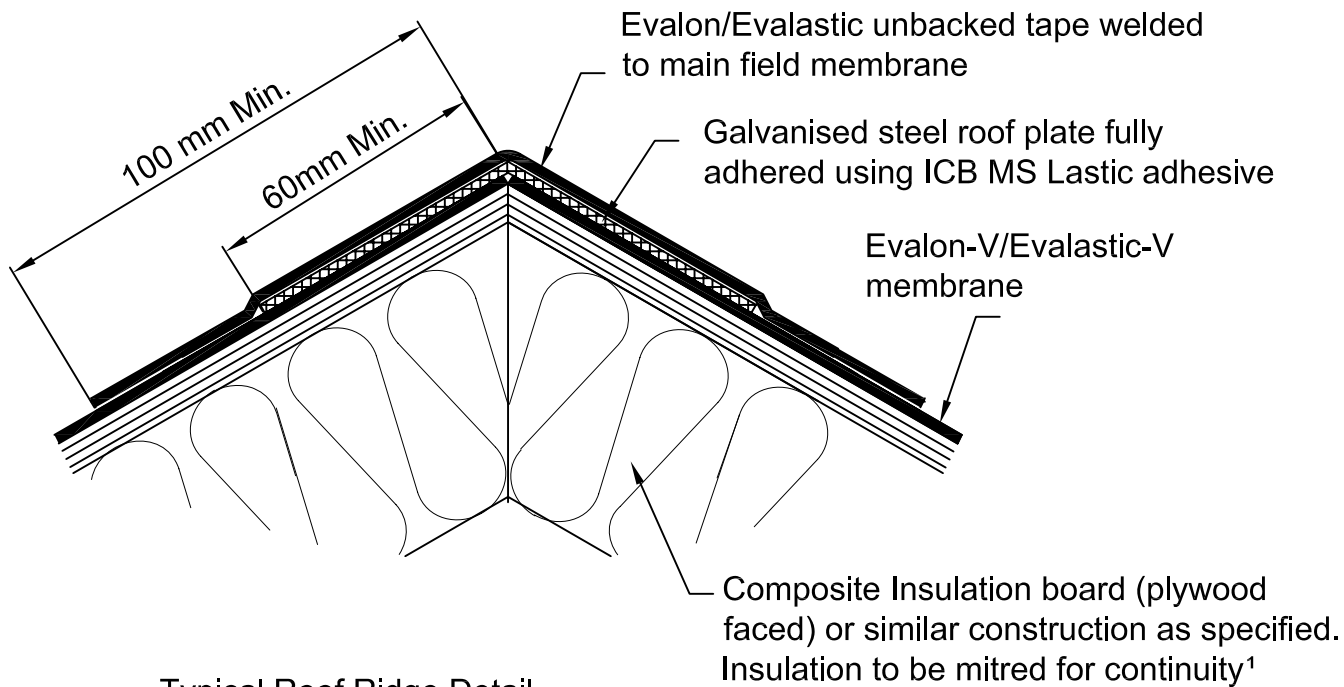
Typical Roof Ridge Detail
